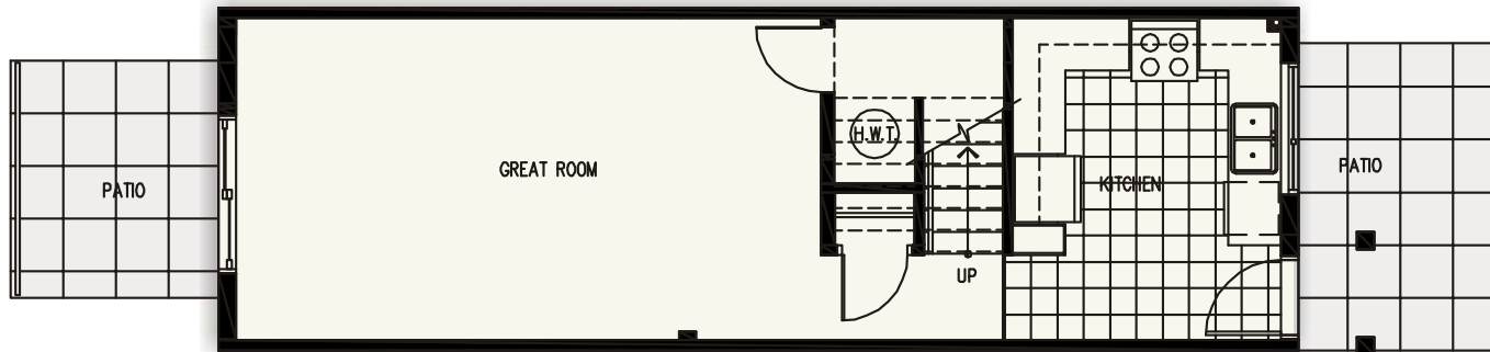
GARDEN LEVEL
